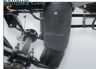
Air suspension bellows
