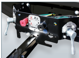
Control panel: front and rear axle separately height-adjustable
